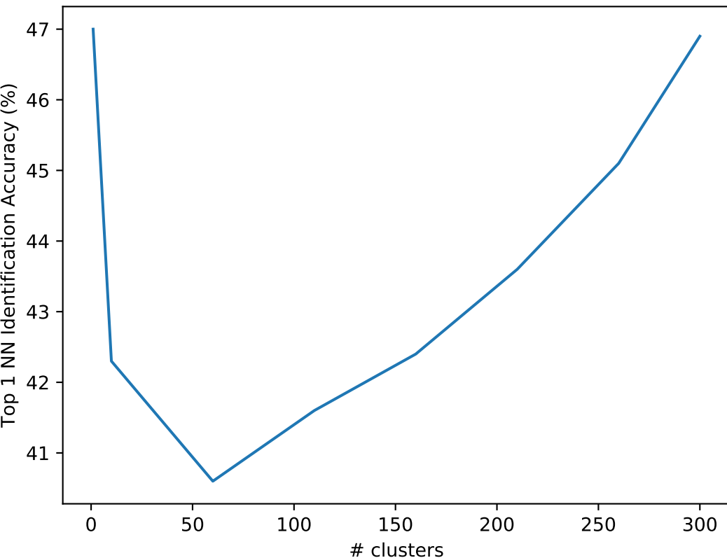
Identification Accuracy varying clusters size
