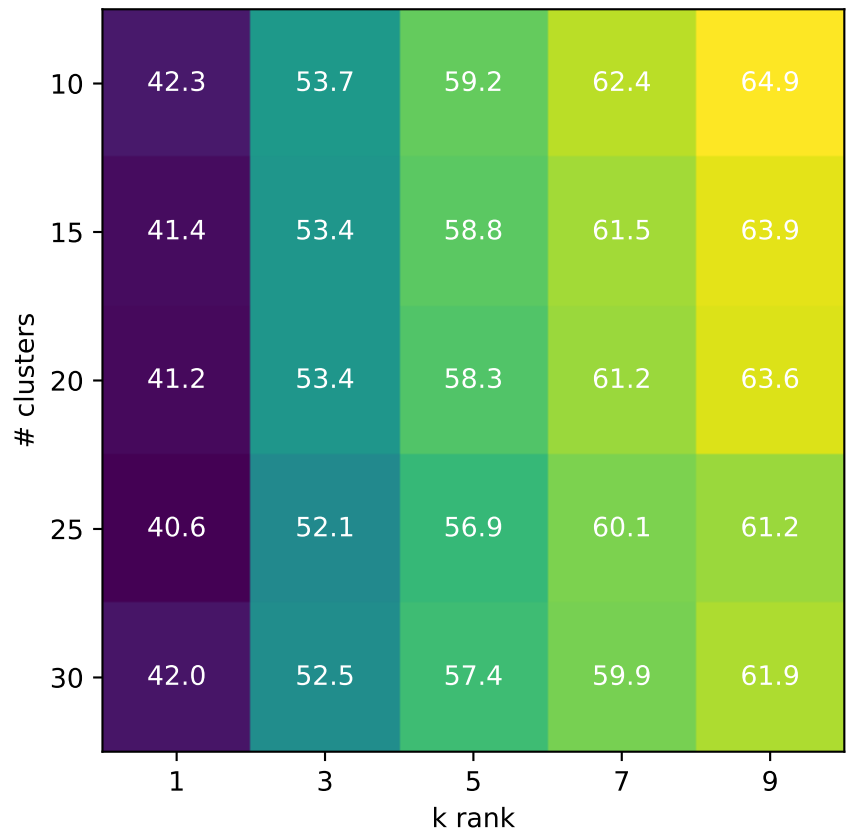
Recognition Accuracy at different k ranks varying number of clusters
