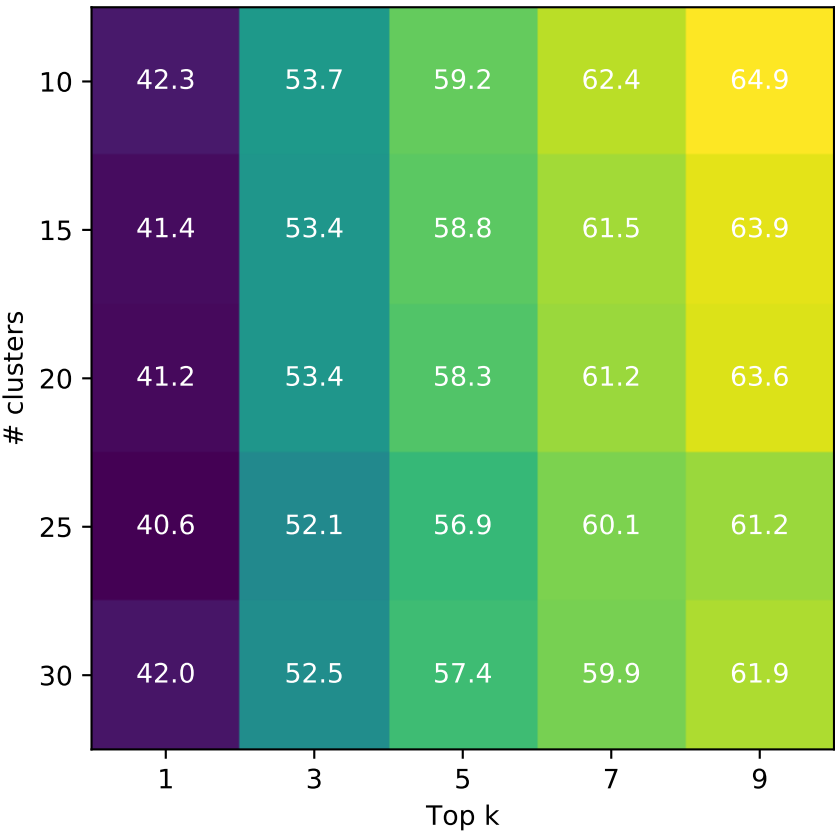
Top k Identification Accuracy for cluster count
