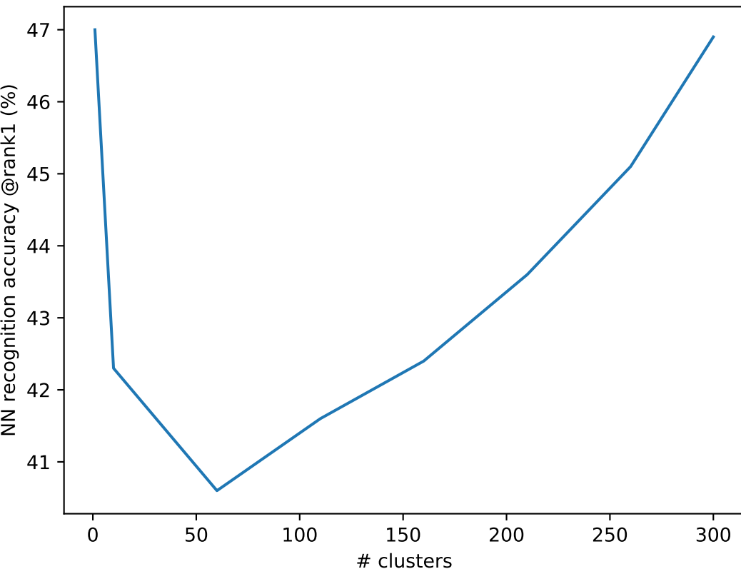
Recognition accuracy varying clusters size
