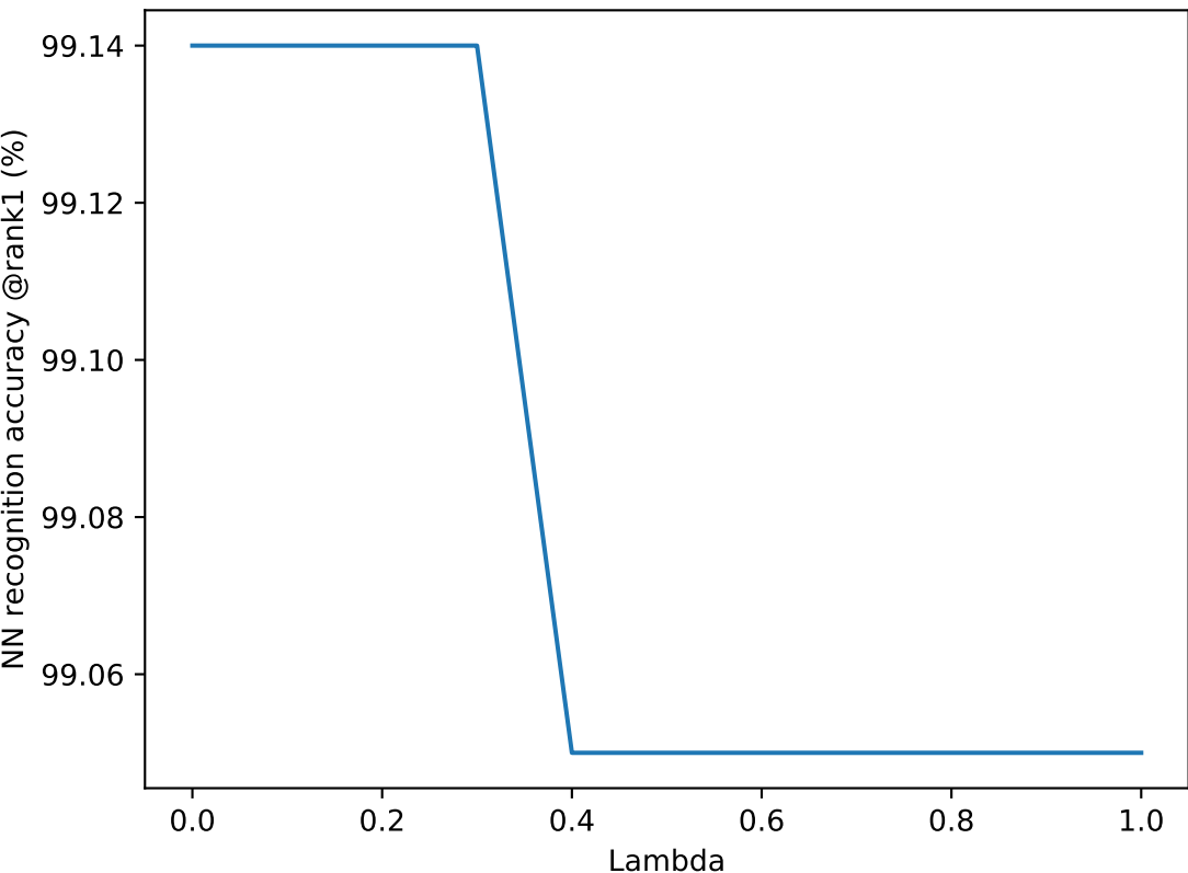
Recognition accuracy varying lambda(training)
