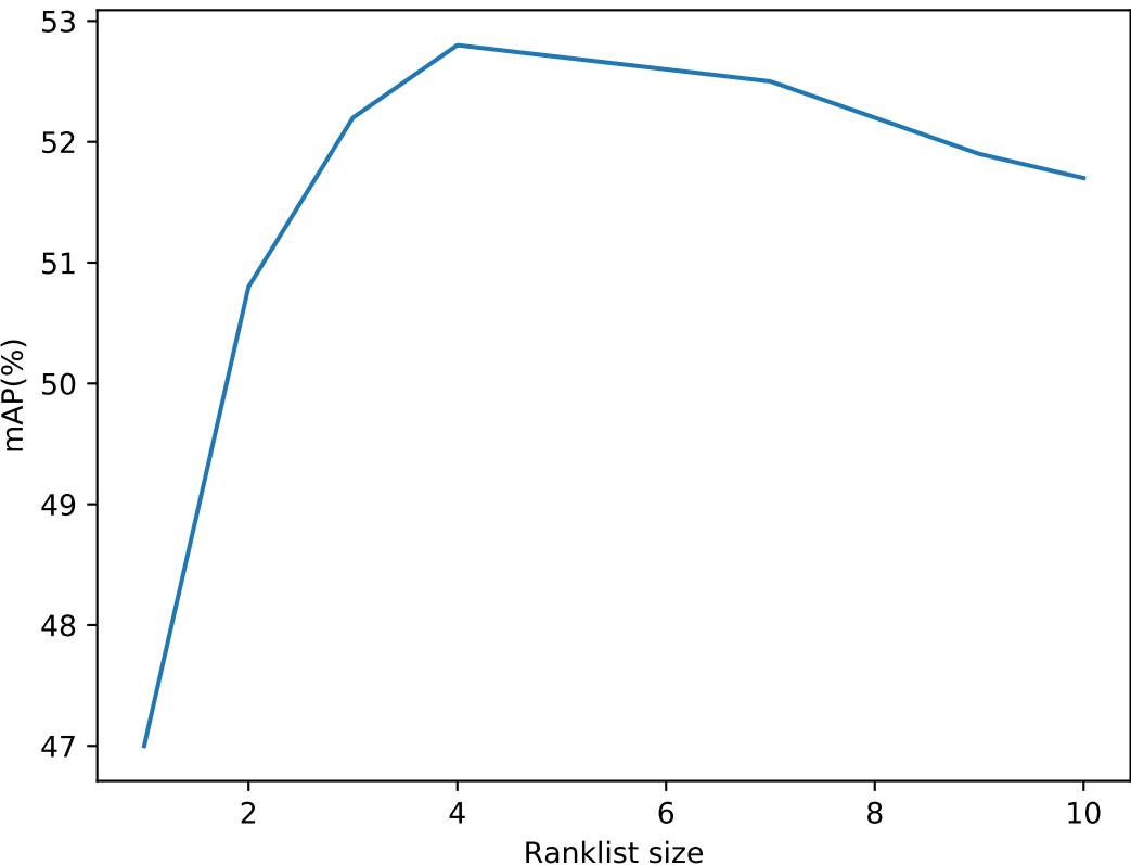
Mean Average Precision
