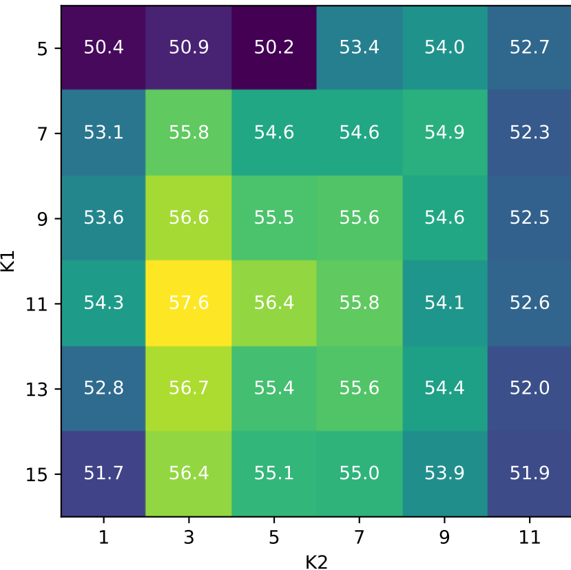
Identification Accuracy varying K1 and K2
