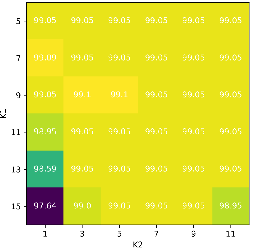
Training Recognition Accuracy varying K1 and K2
