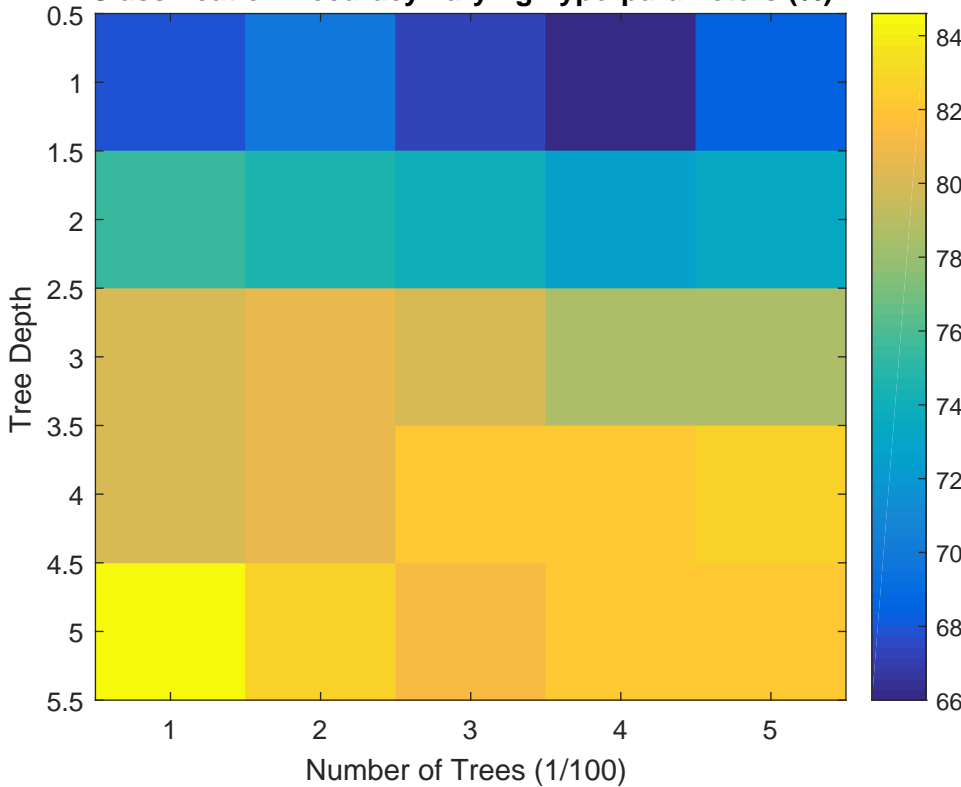
Classification Accuracy varying hyperparameters (%)
