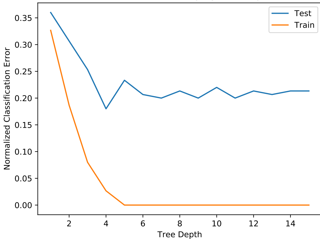
Classification error varying Tree Depth
