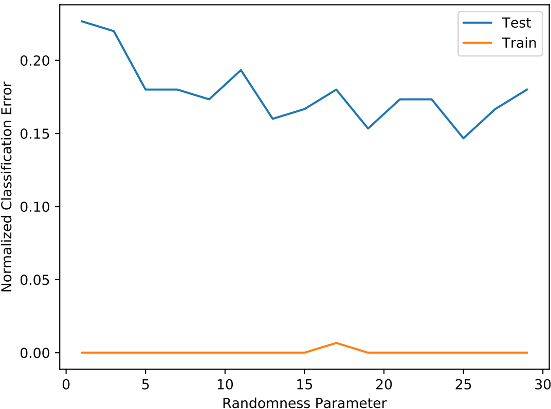
Classification error varying Randomness Parameter
