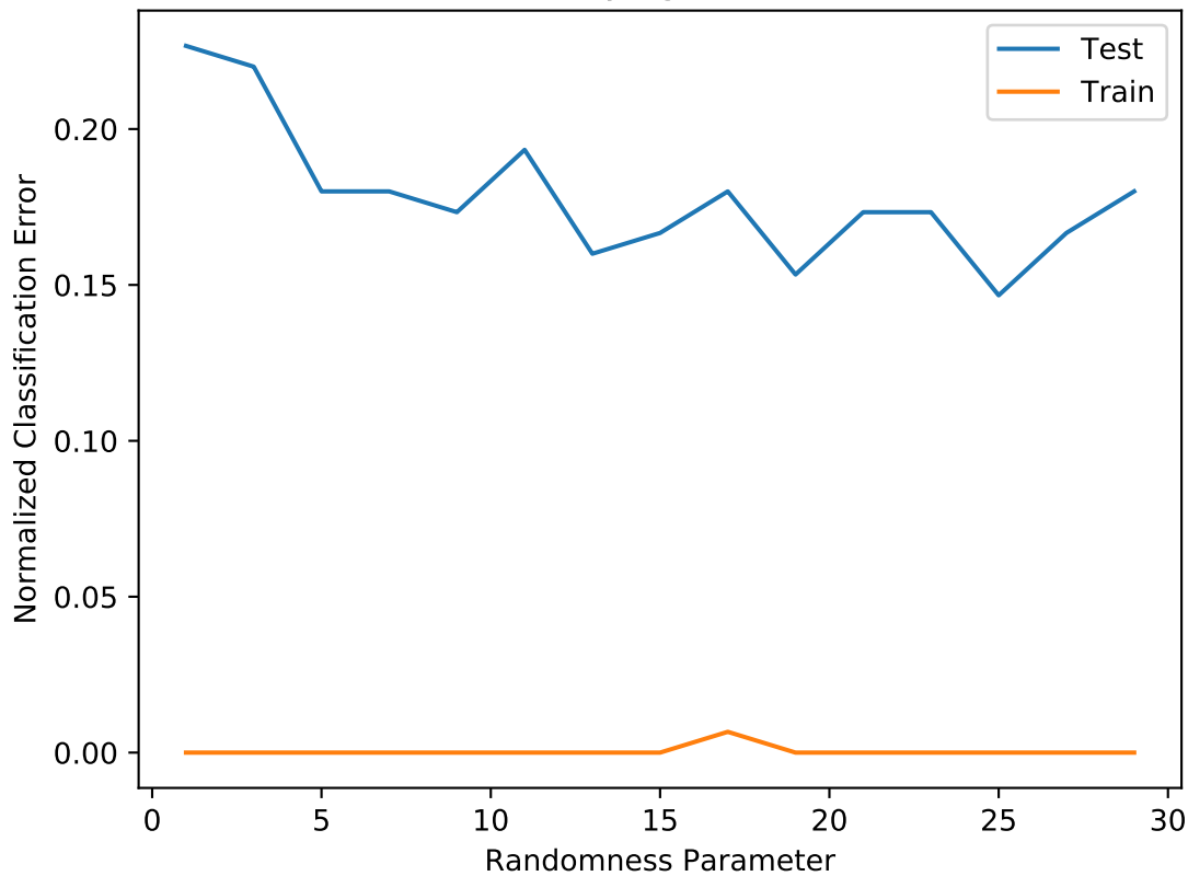
Classification error varying Randomness Parameter
