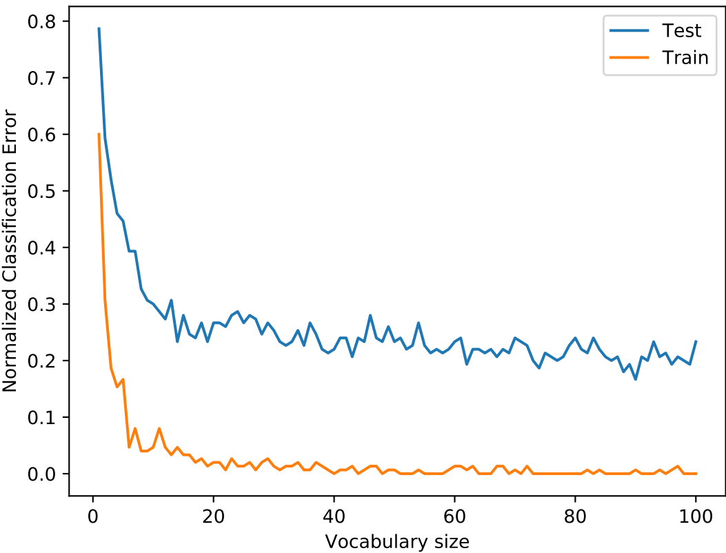
Classification error varying vocabulary size
