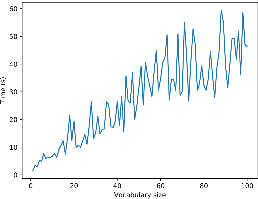
Time complexity varying vocabulary size
